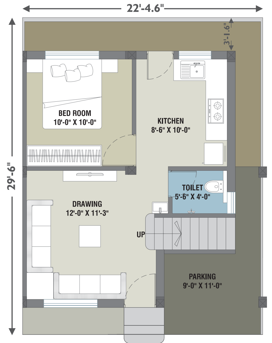
GROUND FLOOR B. AREA 535.64 sq.ft.
