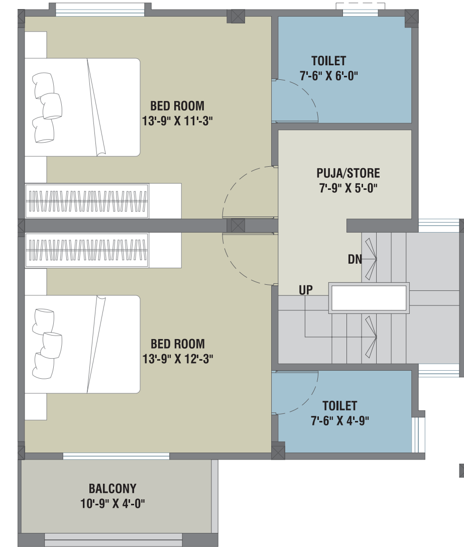
FIRST FLOOR B. AREA 646.931 sq.ft.
