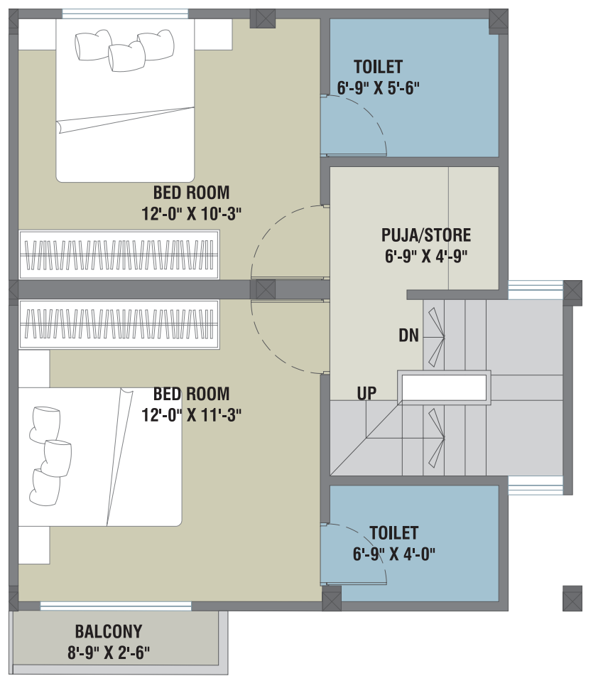
FIRST FLOOR B. AREA 512.39 sq.ft.
